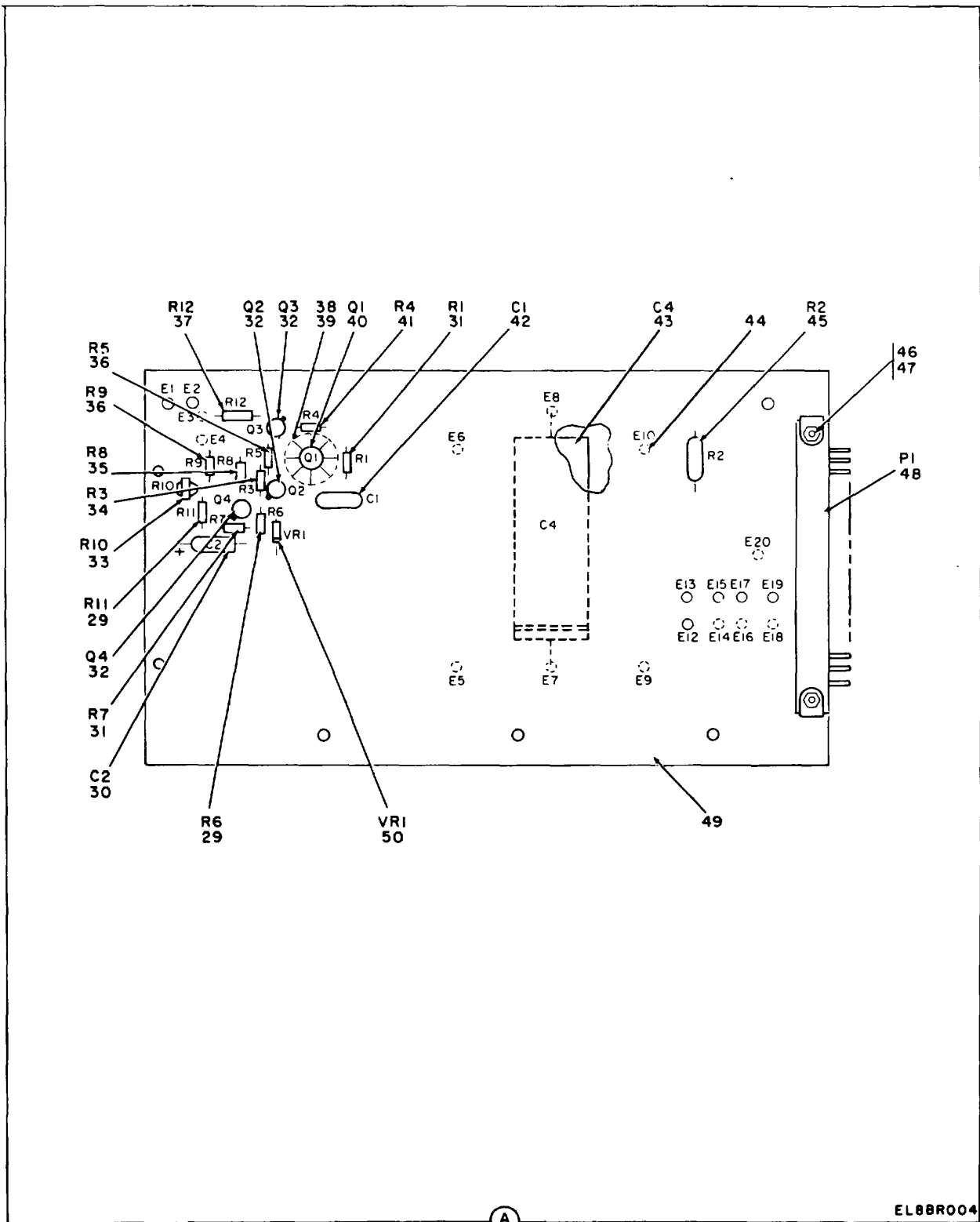
Figure 3. DC Power Supply (Sheet 2 of 2)
